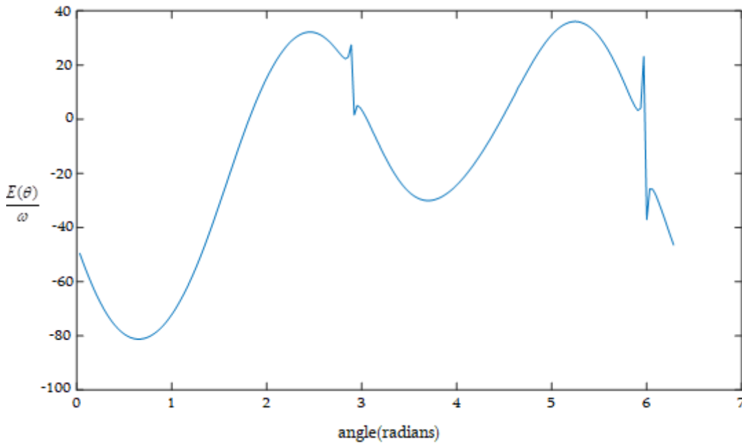
Figure 2: 2-D graph of energy versus angle for \frac{K_3}{\omega} = 21 .
